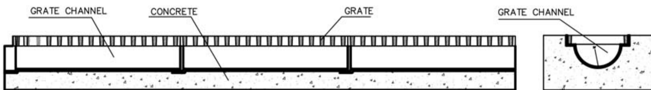
GRATING ASSEMBLY ON GREY CAST IRON CHANNELS IMBEDDED IN CONCRETE
